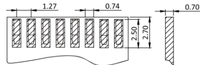
Recommended PCB Layout (PCB TOLERANCE ±0.05)
